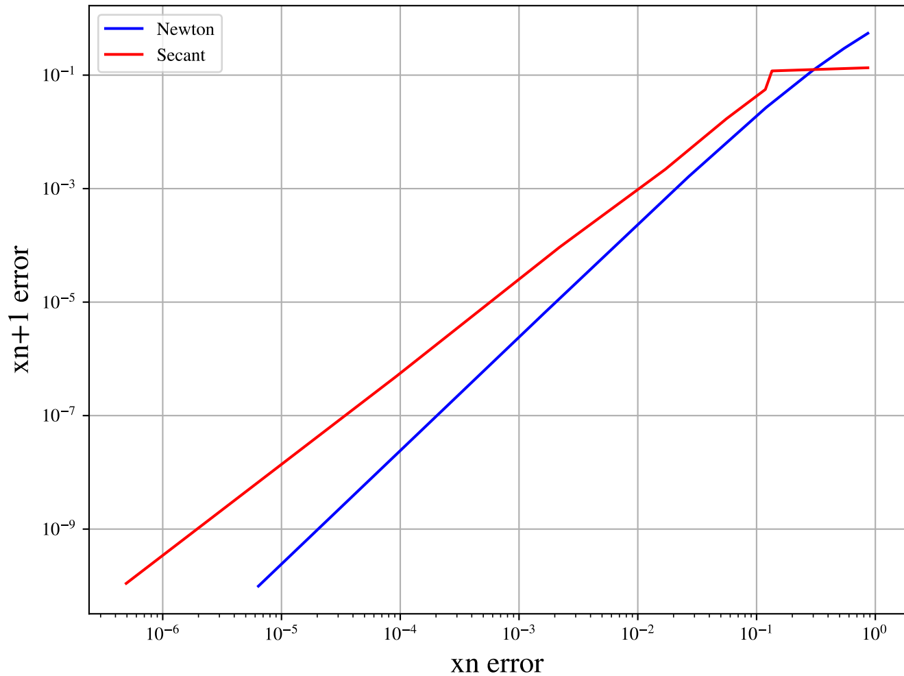
Log Plot of |x_{n+1} - \alpha| vs. |x_n - \alpha|
